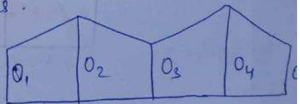
(Trapezoidal rule)
