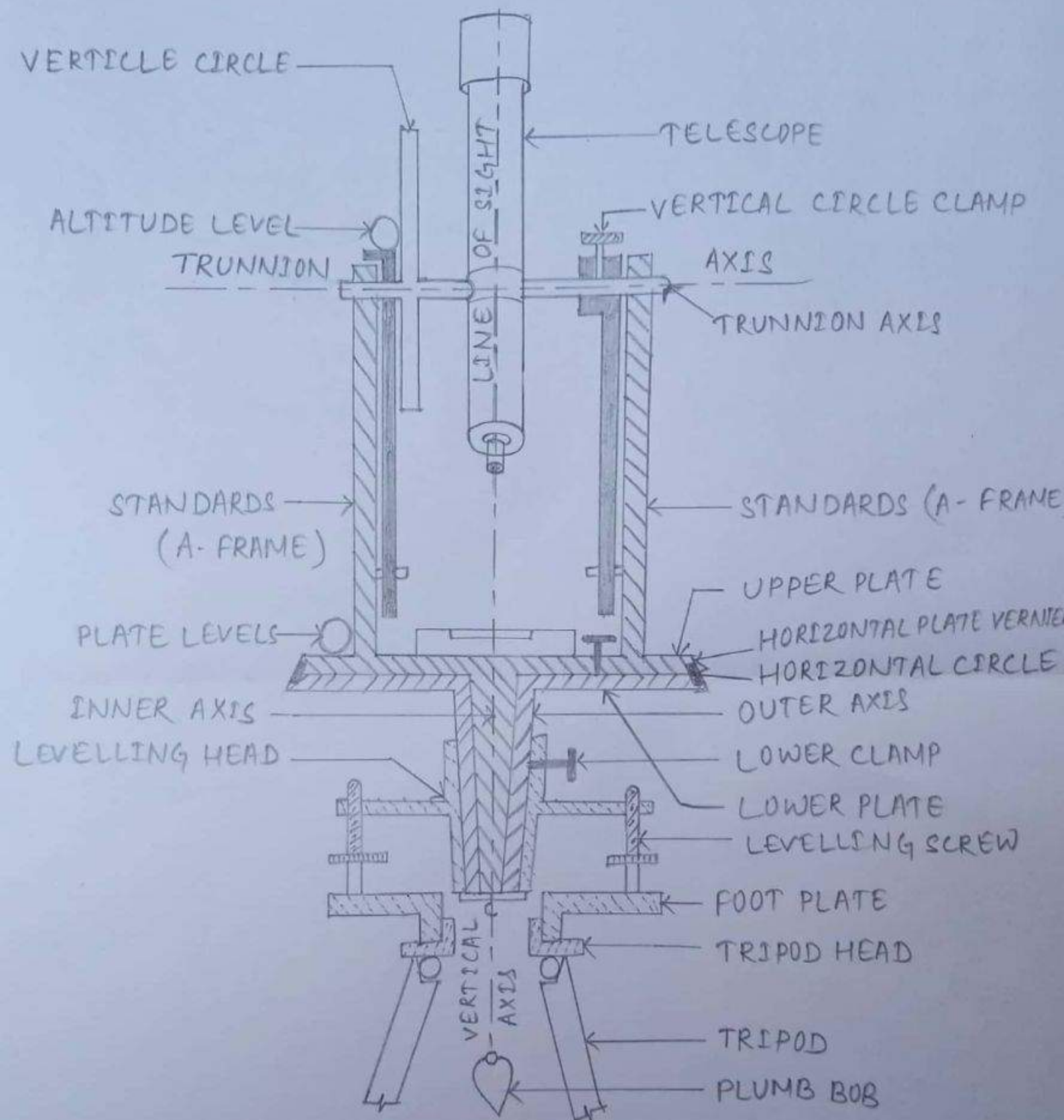
THE ESSENTIALS OF A TRANSIT
