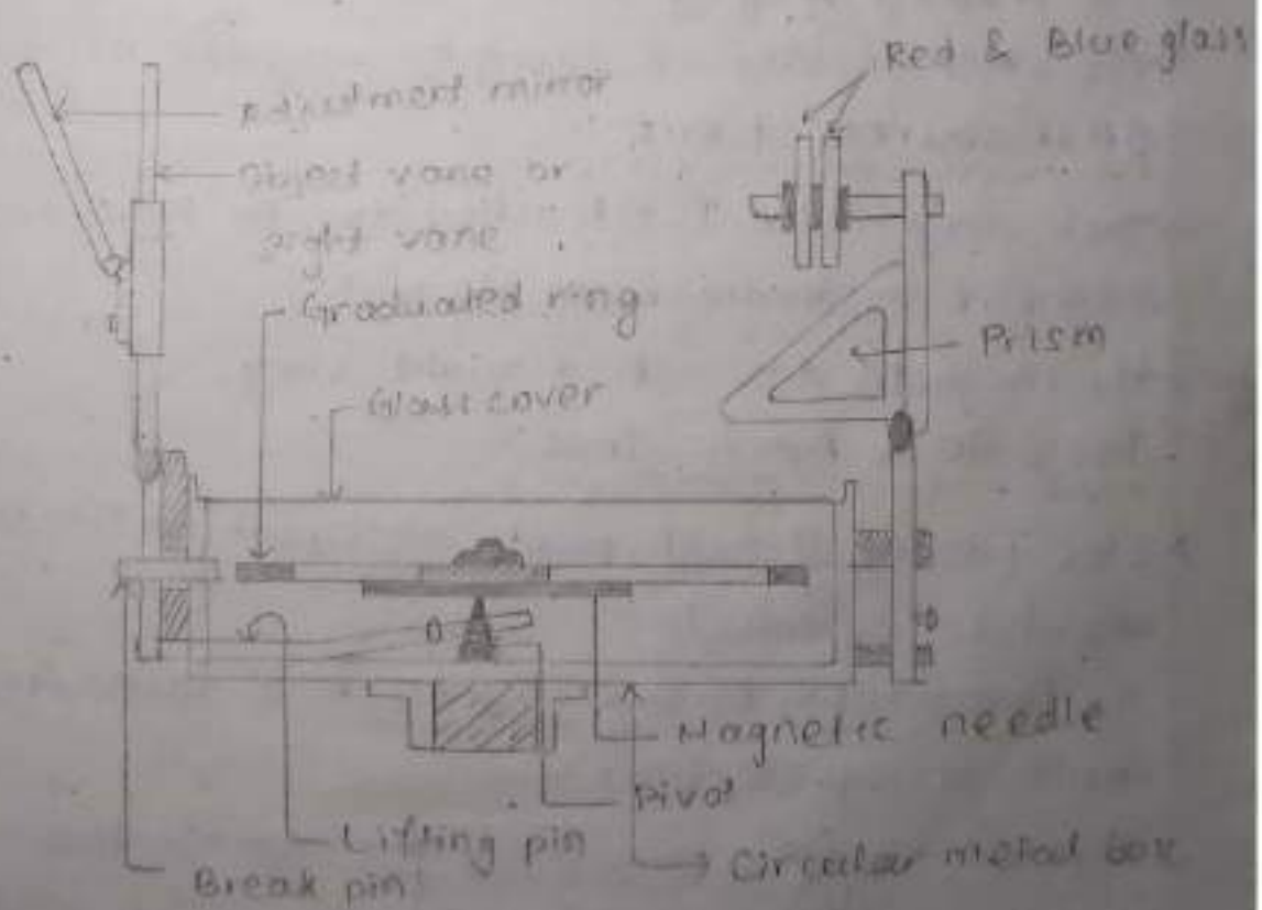
(Prismatic compass)
