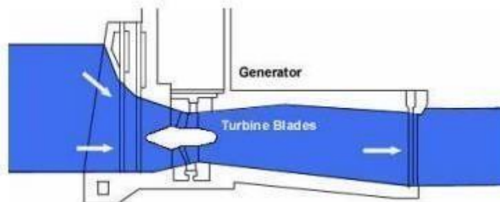
Rim Turbine
