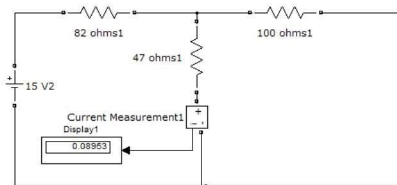
Fig.2: Circuit diagram when V_1 \neq 0 & V_2 = 0
